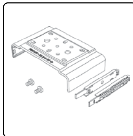
Quick Release Bracket, Guide Rails, Screws
